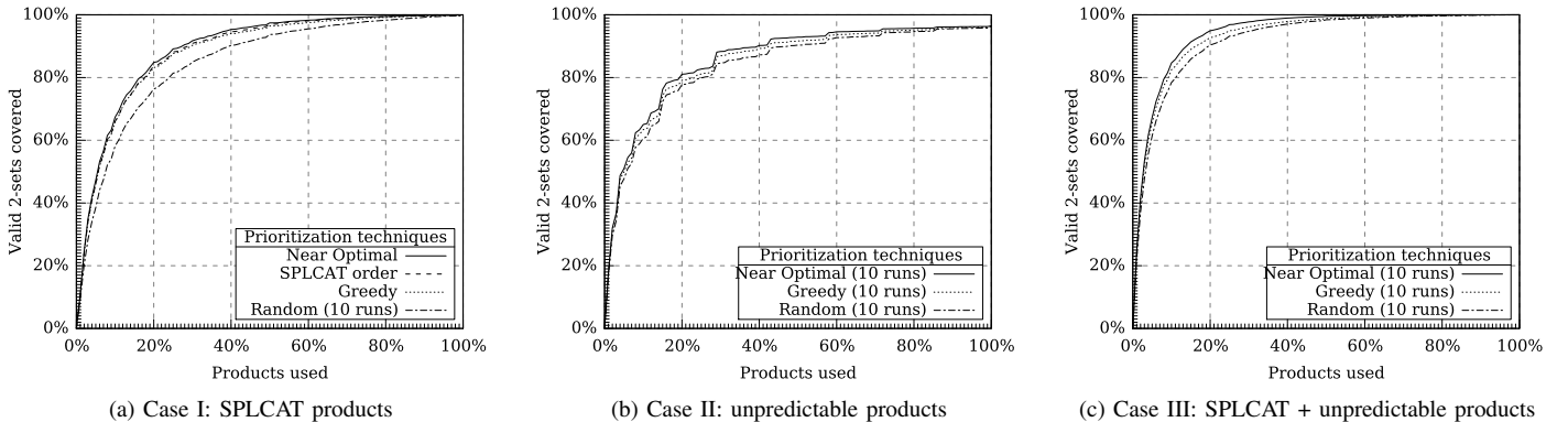
Fig. 3. Prioritization on Moderate FMs ( t = 2 )
